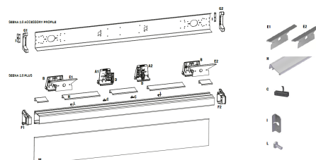
SEENA 2.0 ACCESSORIES AND SPARE PARTS
